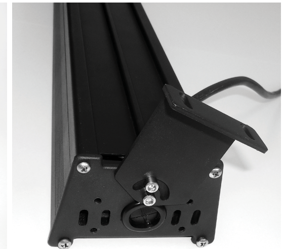
Adjustable mounting bracket kit supplied for installing the fitting at a specific angle
