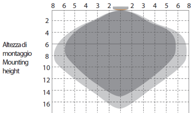
Montaggio soffitto / Ceiling mounted
