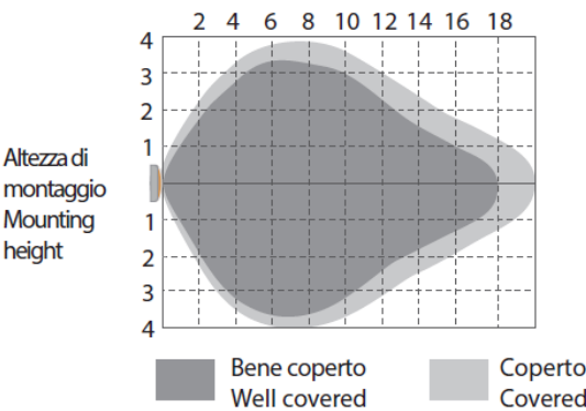
Montaggio parete / Wall mounted
