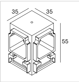
W35/008/W W35/008/B White or black aluminium blind angled joint (1pc)
