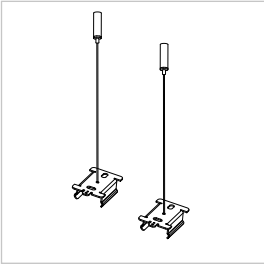
W35/003/SOSP Suspended lighting kits consisting of rose ceiling featuring micro adjustment and L3000mm steel cable (2pcs).
