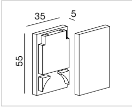
W35/001/W W35/001/B White or black painted aluminium end cap kit (2pcs)
