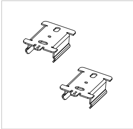
W35/002/CLIP Ceiling installation kit consisting of 2 ceiling fixing clips (dowels and screws not included).
