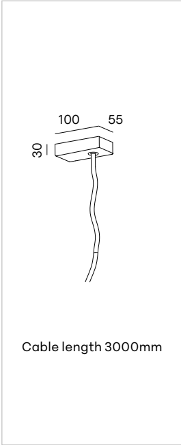
W35/003R/W W35/003R/B White or black 3-pole rose ceiling with power supply kit for on-off drivers.
