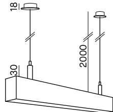
KIT/SOSP/PA Suspension kit for PA/12 (2pz)
