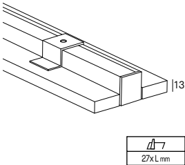
KIT/TRIM/PA12 Trimless kit for PA/12 (2pcs), for plasterboard 13mm depth
