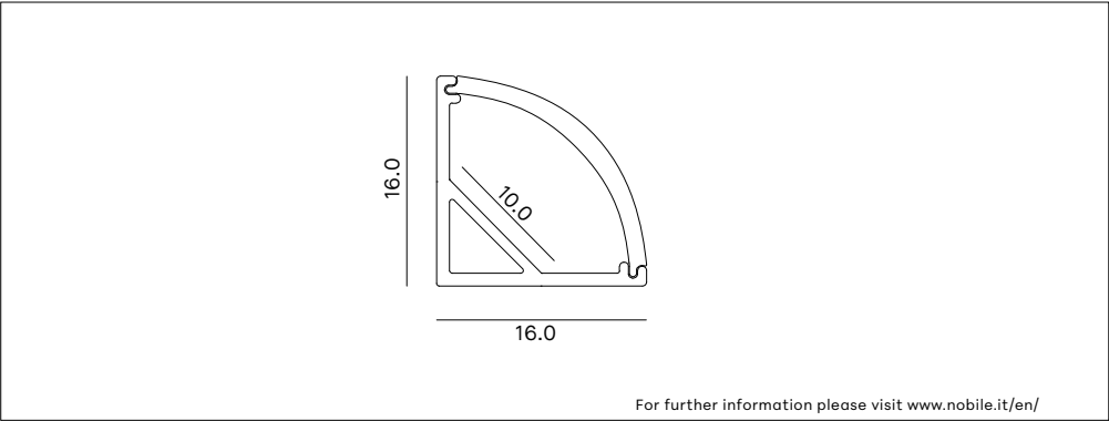
ANGLED SURFACE-MOUNTED ALUMINIUM PROFILE
